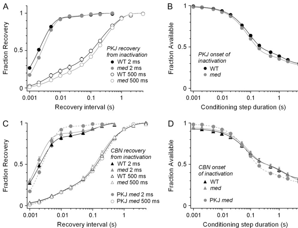
FIGURE 3 Recovery from and entry into inactivated states in wild-type and med neurons. (A and C) Wild-type and med mean fraction of available channels versus recovery interval for (A) Purkinje neurons (2 ms: WT, N = 21 ; med , N = 7 ; 500 ms: WT, N = 13 ; med , N = 7 ) and (C) cerebellar nuclear neurons (2 ms: WT, N = 20 ; med , N = 8 ; 500 ms: WT, N = 17 ; med , N = 5 ). Channels recovered from a 2-ms step according to a double exponential and from a 500-ms step according to a triple exponential. Parameters of the fits are given in Table 1. Gray circles in C are the data from med Purkinje neurons, for comparison. For some data points, error bars are smaller than the symbols. (B and D) Wild-type and med average fraction of available channels versus conditioning pulse interval for (B) Purkinje neurons (WT, N = 12 ; med , N = 8 ) and (D) cerebellar nuclear neurons (WT, N = 15 ; med , N = 5 ). Channels entered slow-inactivated states in two phases (Table 1). Gray circles in D are the data from med Purkinje neurons, for comparison. For some data points, error bars are smaller than the symbols.
